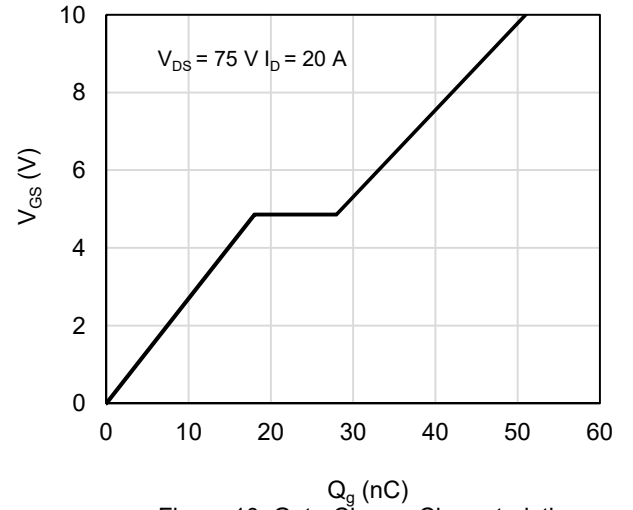
Figure 10: Gate-Charge Characteristics
